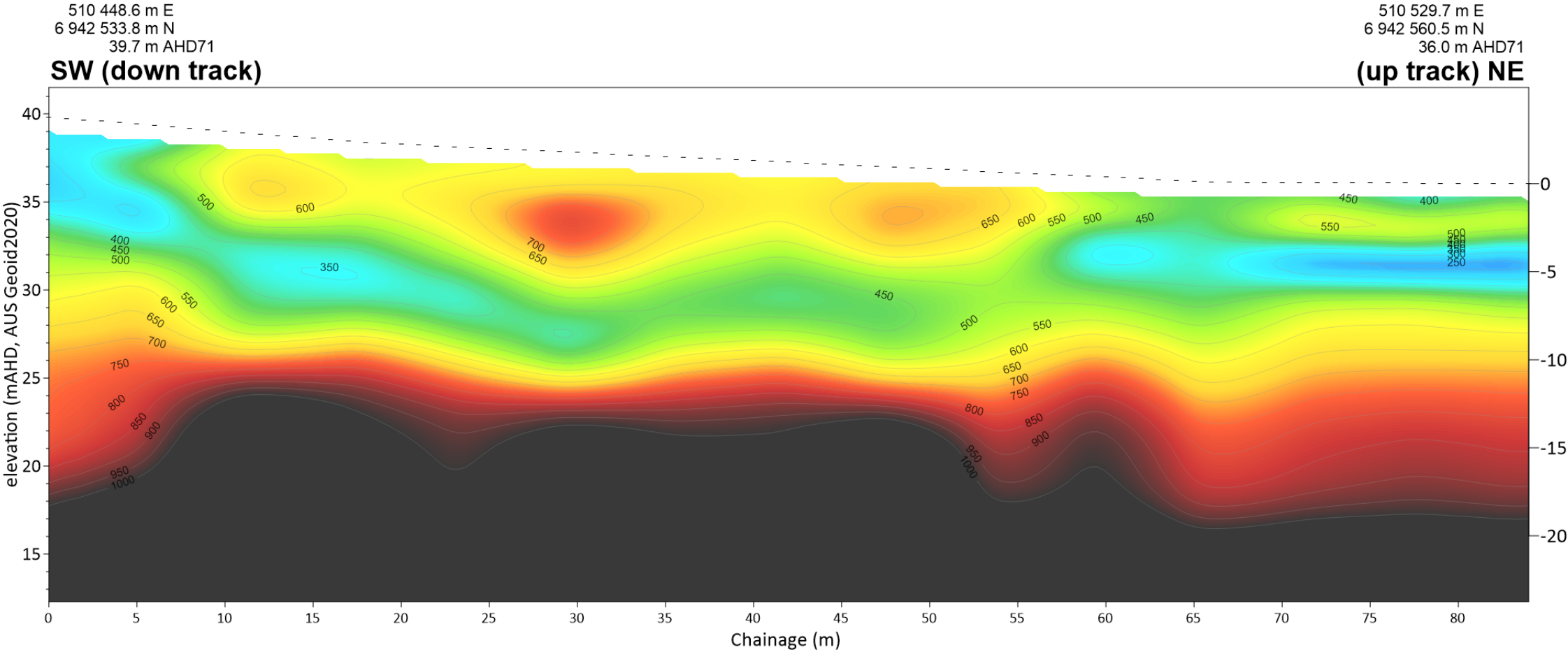
Seismic Line MASW AU-GP 136
